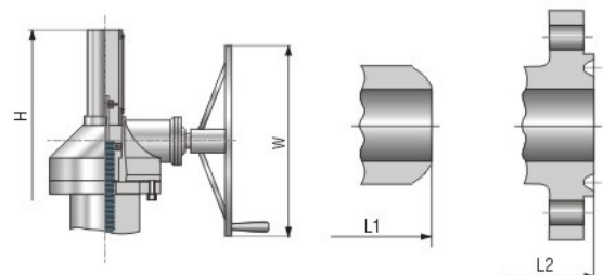
• Gear operation for 14" and larger BW End RTJ End
